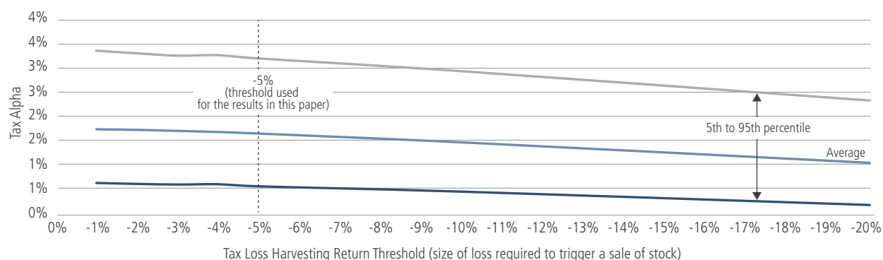
FIGURE 5. SIMULATED TAX ALPHA DIMINISHES AS THE TAX LOSS HARVESTING RETURN THRESHOLD IS MADE MORE NEGATIVE
